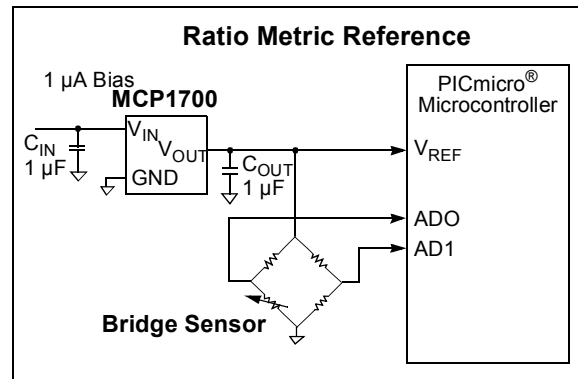
FIGURE 6-2: Using the MCP1700 as a voltage reference.
